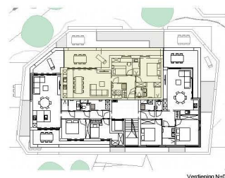
Verdieping N+02
